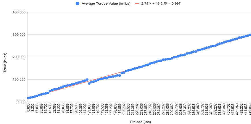
Torque VS. Preload
