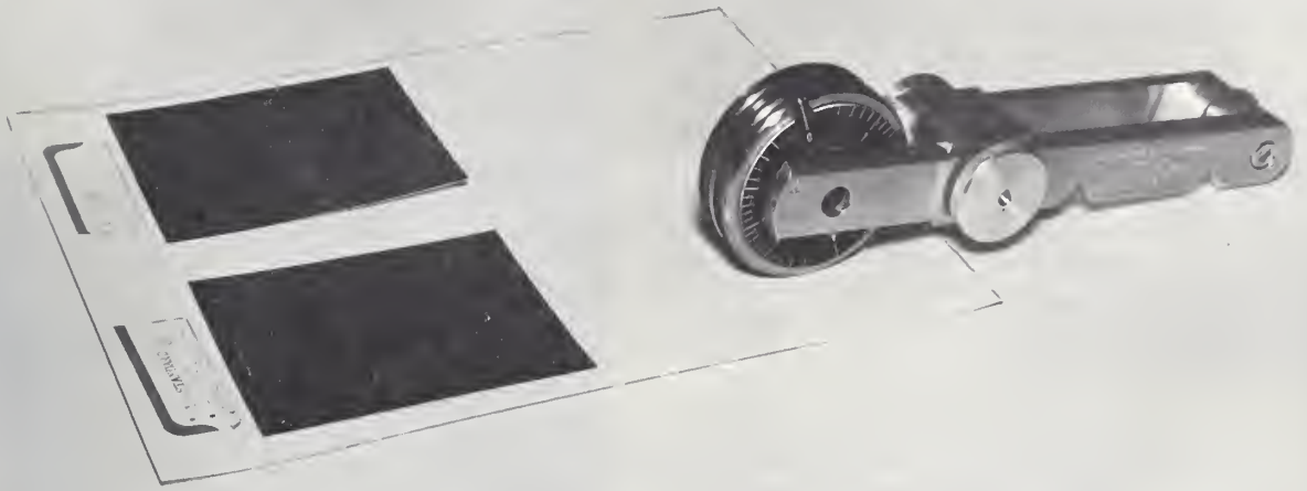
FIGURE 7.3. Interchemical wet film thickness gage, with holder; when gage is rolled over wet surface, thickness is indicated by point of first contact of paint with recessed, eccentric, calibrated inner wheel, as described in ASTM Method D 1212-54 (also, see text, p. 137). (Photo courtesy of Gardner Laboratory.)
