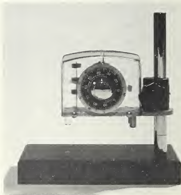
FIGURE 7.2. Magne-Gage measures thickness of non-magnetic coatings on magnetic (ferrous) substrates (see text, p. 138) as described in ASTM Method D 1186-53.
