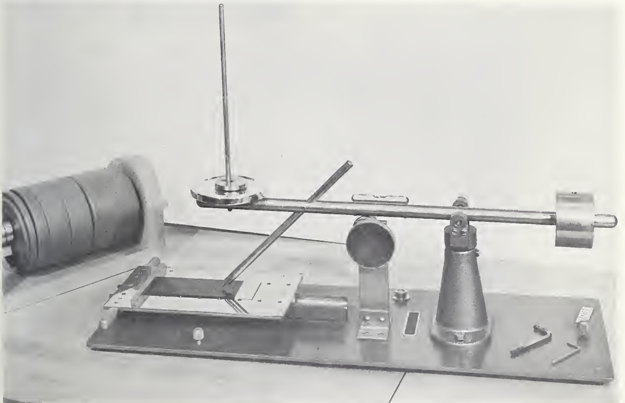
FIGURE 7.4. Balanced-beam scrape-adhesion tester determines load required to remove coating with U-shaped stylus, as described in ASTM Method D 2197-63T.
