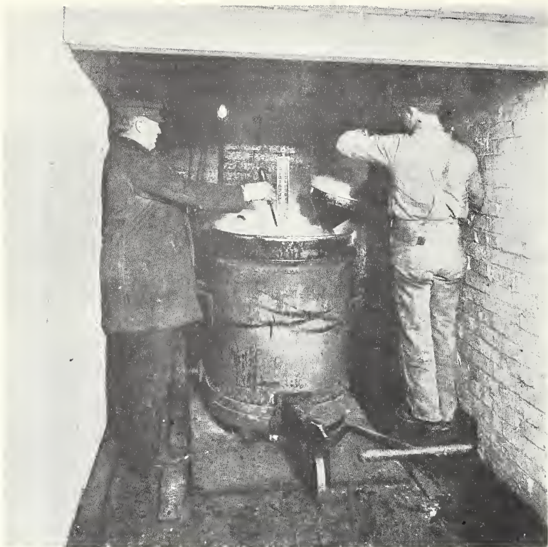
FIGURE 1.1. Early varnish-making; putting in the oil. (Bottler, M., and A. H. Sabin, German and American varnish making , John Wiley & Sons, New York, N. Y. 10016, 1912.)
