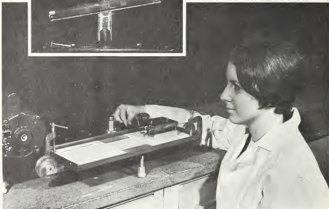
FIGURE 2.5. Washability machine for measuring scrub resistance of paints as described in ASTM Method D 2486-66T.
